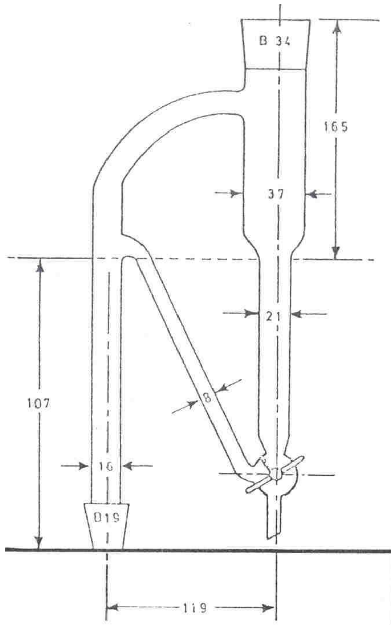
Diagram of a modified Cleveger-type separator
