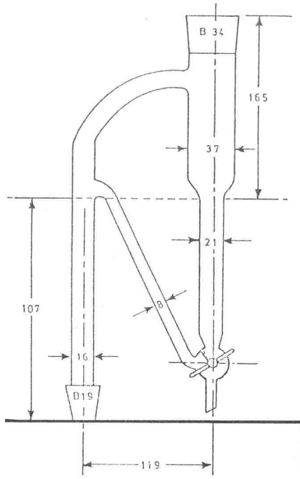
Diagram of a modified Cleveger-type separator
